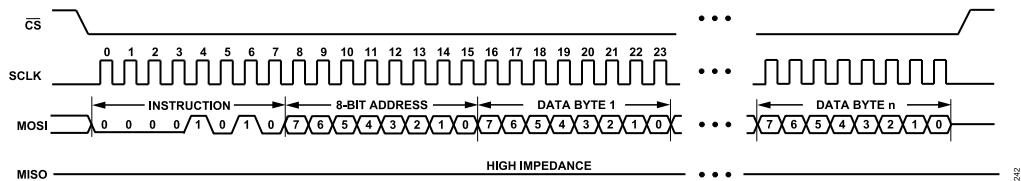
Figure 39. Burst Write (Receive Instruction Only)
