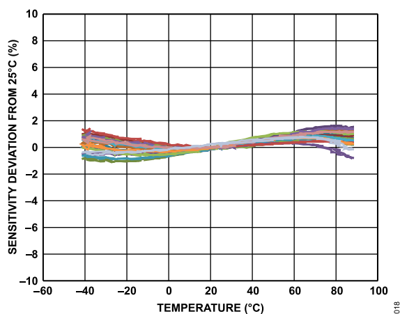
Figure 18. Y-Axis Sensitivity Deviation from 25°C vs. Temperature— 16 Parts Soldered to PCB, ODR = 100 Hz, V_S = 2 V
