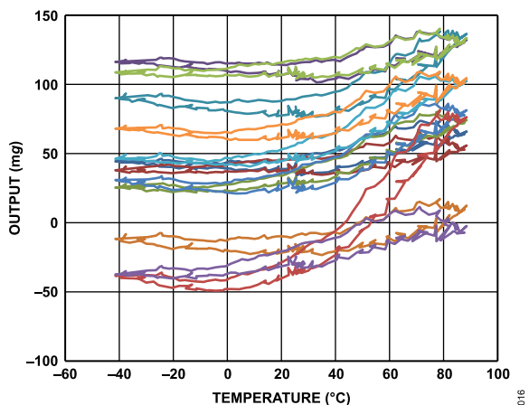
Figure 16. Z-Axis Zero g Offset vs. Temperature— 16 Parts Soldered to PCB, ODR = 100 Hz, V_S = 2\text{ V}
