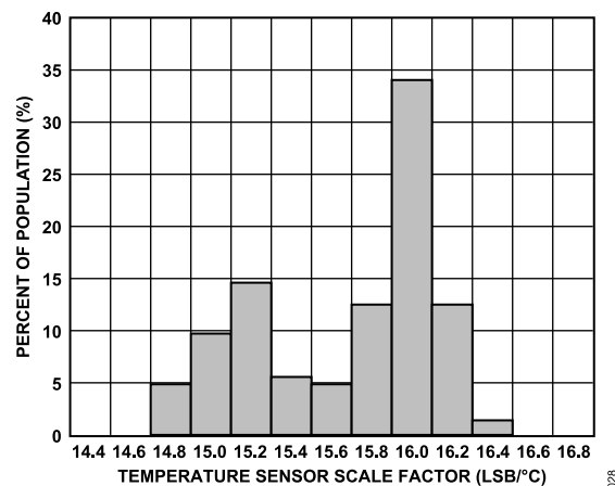
Figure 28. Temperature Sensor Scale Factor, V_S = 2\text{ V}
