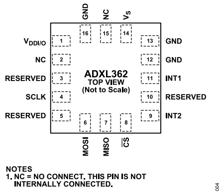
Figure 4. Pin Configuration (Top View)
