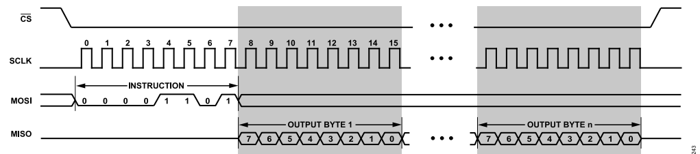
Figure 40. FIFO Read
