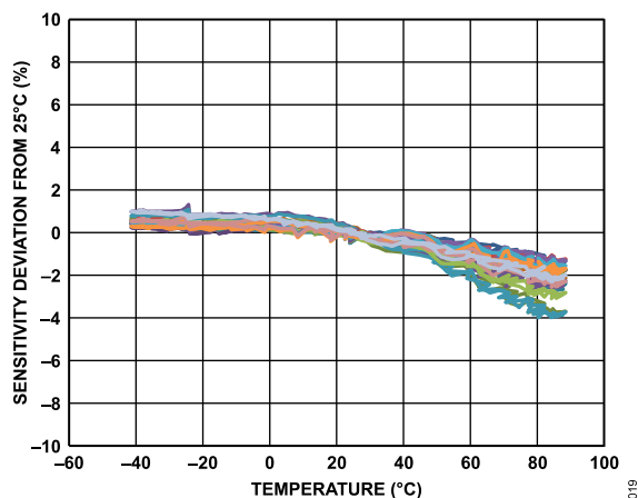
Figure 19. Z-Axis Sensitivity Deviation from 25°C vs. Temperature— 16 Parts Soldered to PCB, ODR = 100 Hz, V_S = 2 V
