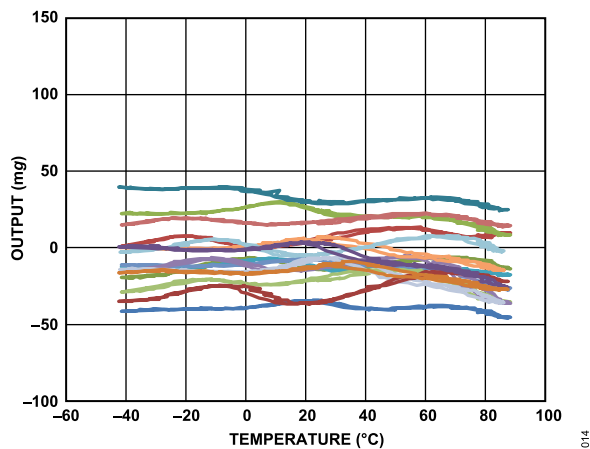
Figure 14. X-Axis Zero g Offset vs. Temperature— 16 Parts Soldered to PCB, ODR = 100 Hz, V_S = 2\text{ V}
