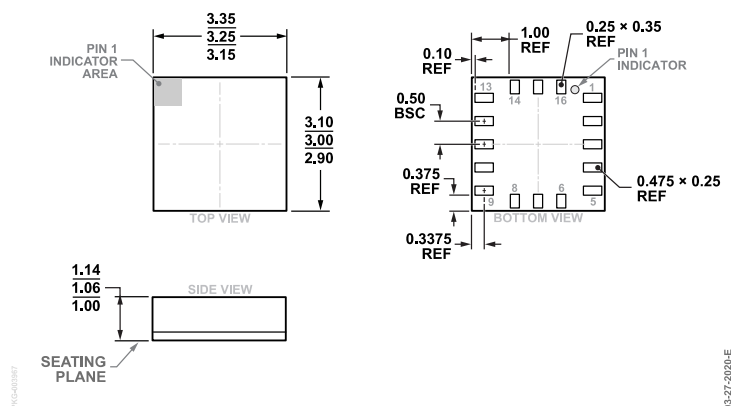
Figure 54. 16-Terminal Land Grid Array [LGA] (CC-16-4) Dimensions Shown in Millimeters
