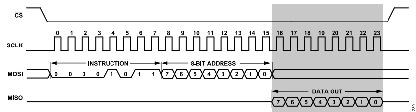
Figure 36. Register Read
