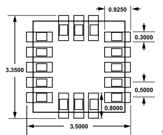
Figure 53. Recommended PCB Land Pattern (Dimensions Shown in Millimeters)
