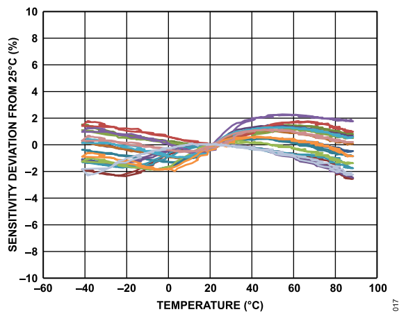
Figure 17. X-Axis Sensitivity Deviation from 25°C vs. Temperature— 16 Parts Soldered to PCB, ODR = 100 Hz, V_S = 2 V
