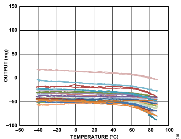
Figure 15. Y-Axis Zero g Offset vs. Temperature— 16 Parts Soldered to PCB, ODR = 100 Hz, V_S = 2\text{ V}
