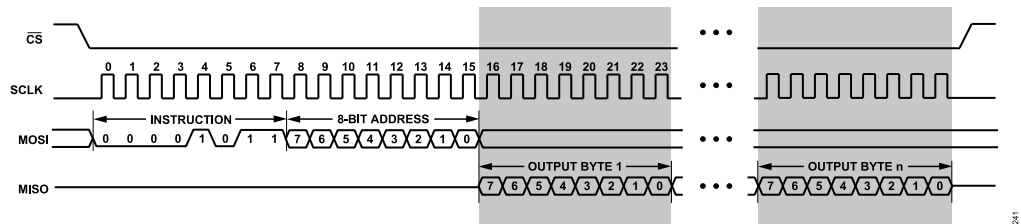
Figure 38. Burst Read
