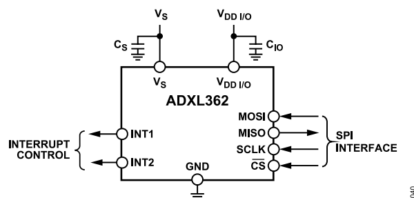
Figure 46. Recommended Bypass Capacitors
